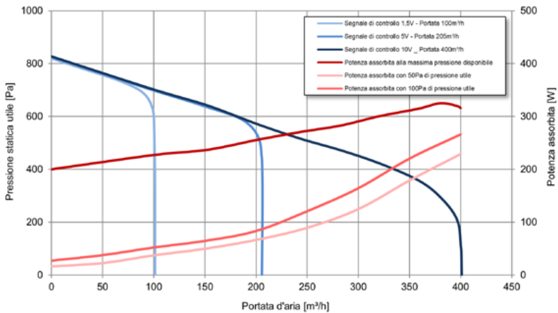
Diagramma prestazioni aerauliche Ventiza EDU UV3-400S / UVE-400S
