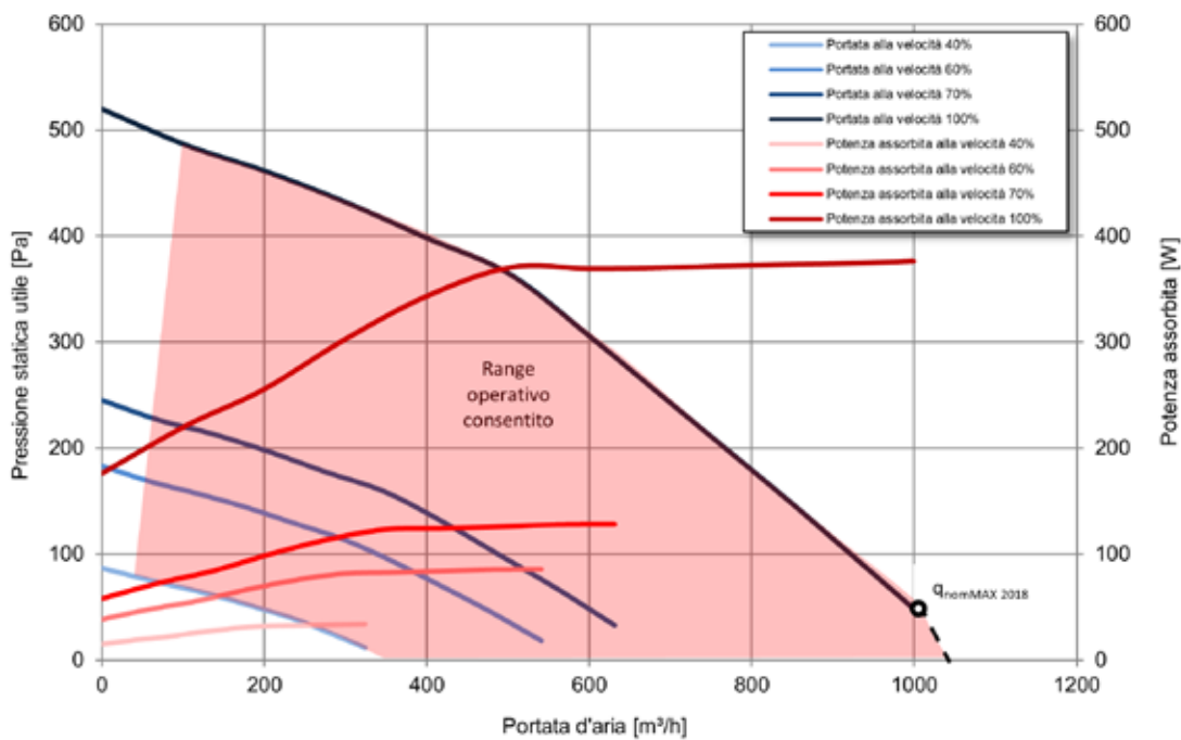
Diagramma prestazioni aerauliche Ventiza EDU UV3-920S / UVE-920S
