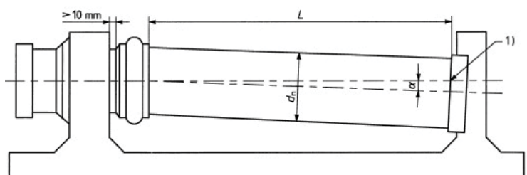
Figure 2: APOLLO Pipes Flexibility Test
